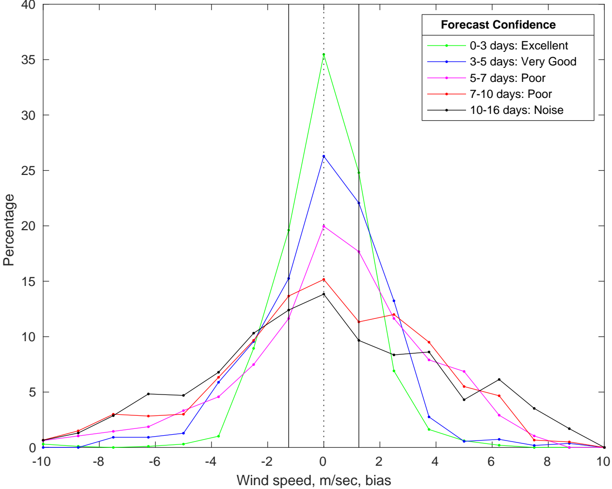
NDBC 42019 vs GFS Winds Bias Histogram: 21-Jan-2026
