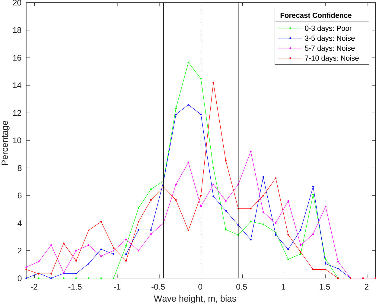
NDBC 42020 vs CMEMS Waves Bias Histogram: 21-Jan-2026
