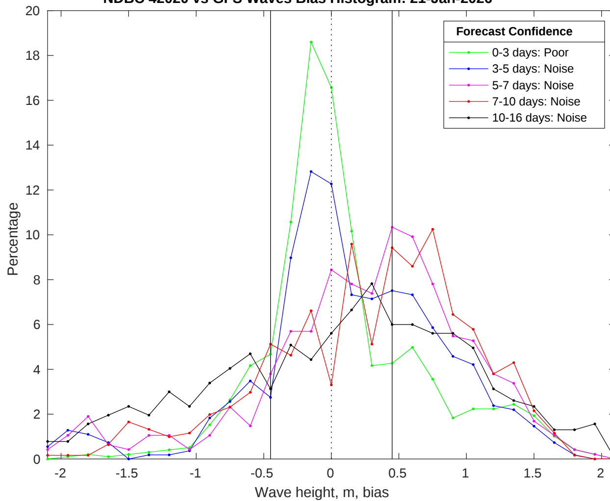
NDBC 42020 vs GFS Waves Bias Histogram: 21-Jan-2026
