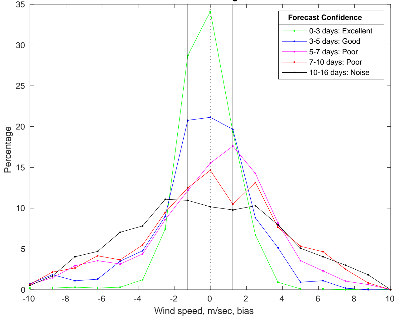
NDBC 42020 vs GFS Winds Bias Histogram: 21-Jan-2026
