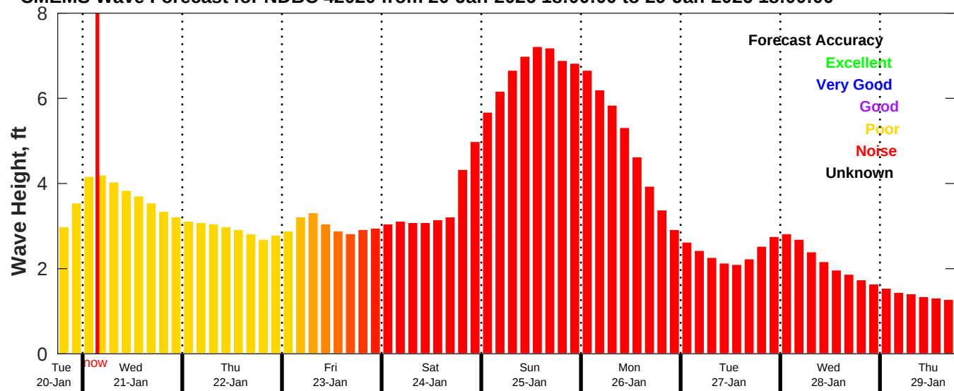
CMEMS Wave Forecast for NDBC 42020 from 20-Jan-2026 18:00:00 to 29-Jan-2026 18:00:00
