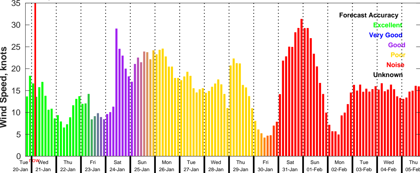
GFS Wind Speed Forecast for NDBC 42020 from 20-Jan-2026 18:00:00 to 05-Feb-2026 18:00:00
