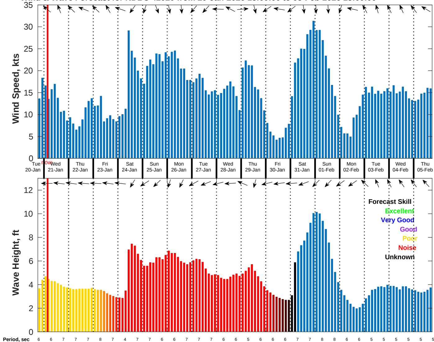
Wind & Wave Forecast for NDBC 42020 from 20-Jan-2026 18:00:00 to 05-Feb-2026 18:00:00
