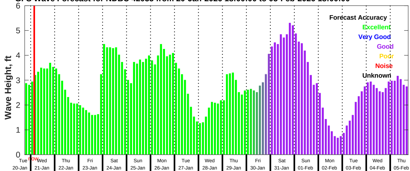
GFS Wave Forecast for NDBC 42035 from 20-Jan-2026 18:00:00 to 05-Feb-2026 18:00:00
