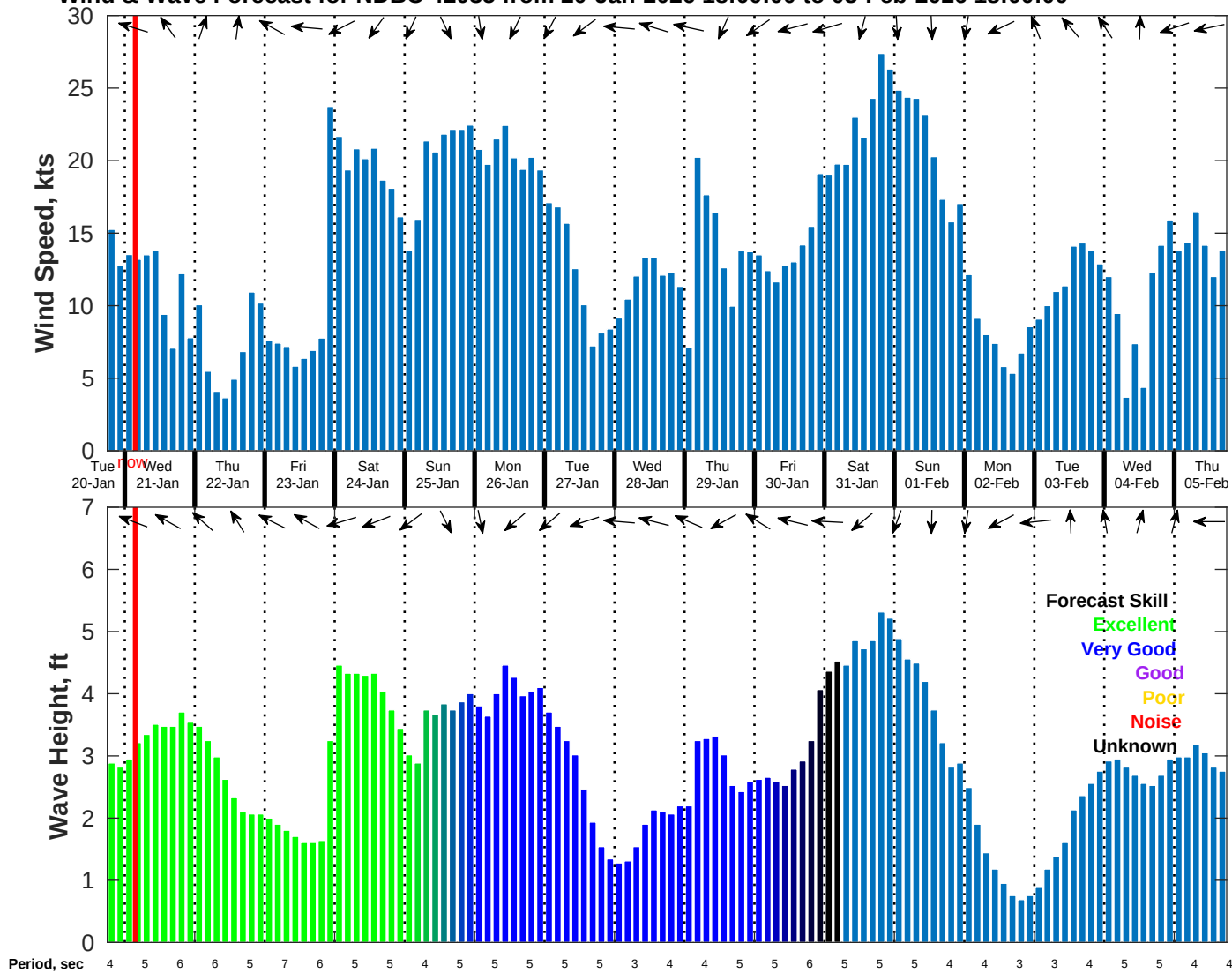
Wind & Wave Forecast for NDBC 42035 from 20-Jan-2026 18:00:00 to 05-Feb-2026 18:00:00
