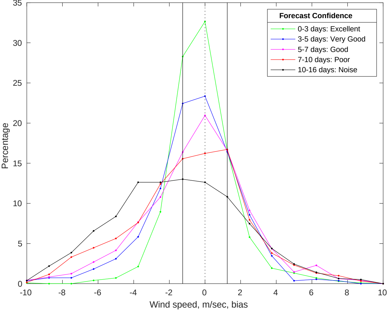
NDBC 42036 vs GFS Winds Bias Histogram: 21-Jan-2026
