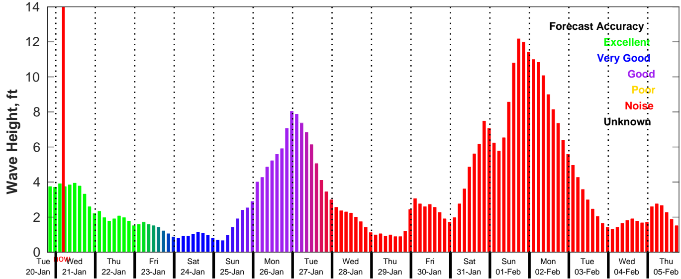
GFS Wave Forecast for NDBC 42036 from 20-Jan-2026 19:00:00 to 05-Feb-2026 19:00:00
