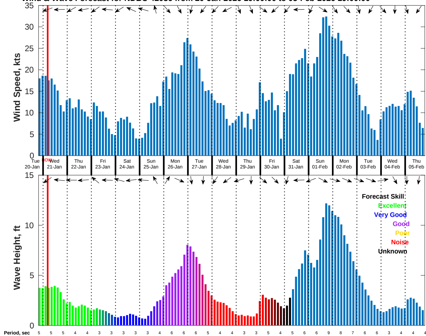
Wind & Wave Forecast for NDBC 42036 from 20-Jan-2026 19:00:00 to 05-Feb-2026 19:00:00
