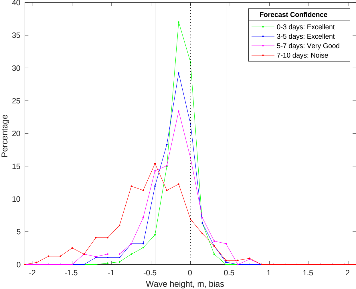
NDBC 42040 vs CMEMS Waves Bias Histogram: 21-Jan-2026
