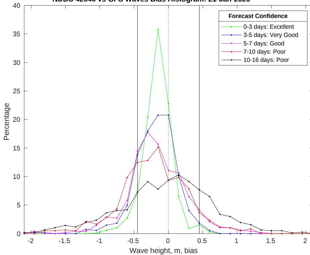
NDBC 42040 vs GFS Waves Bias Histogram: 21-Jan-2026
