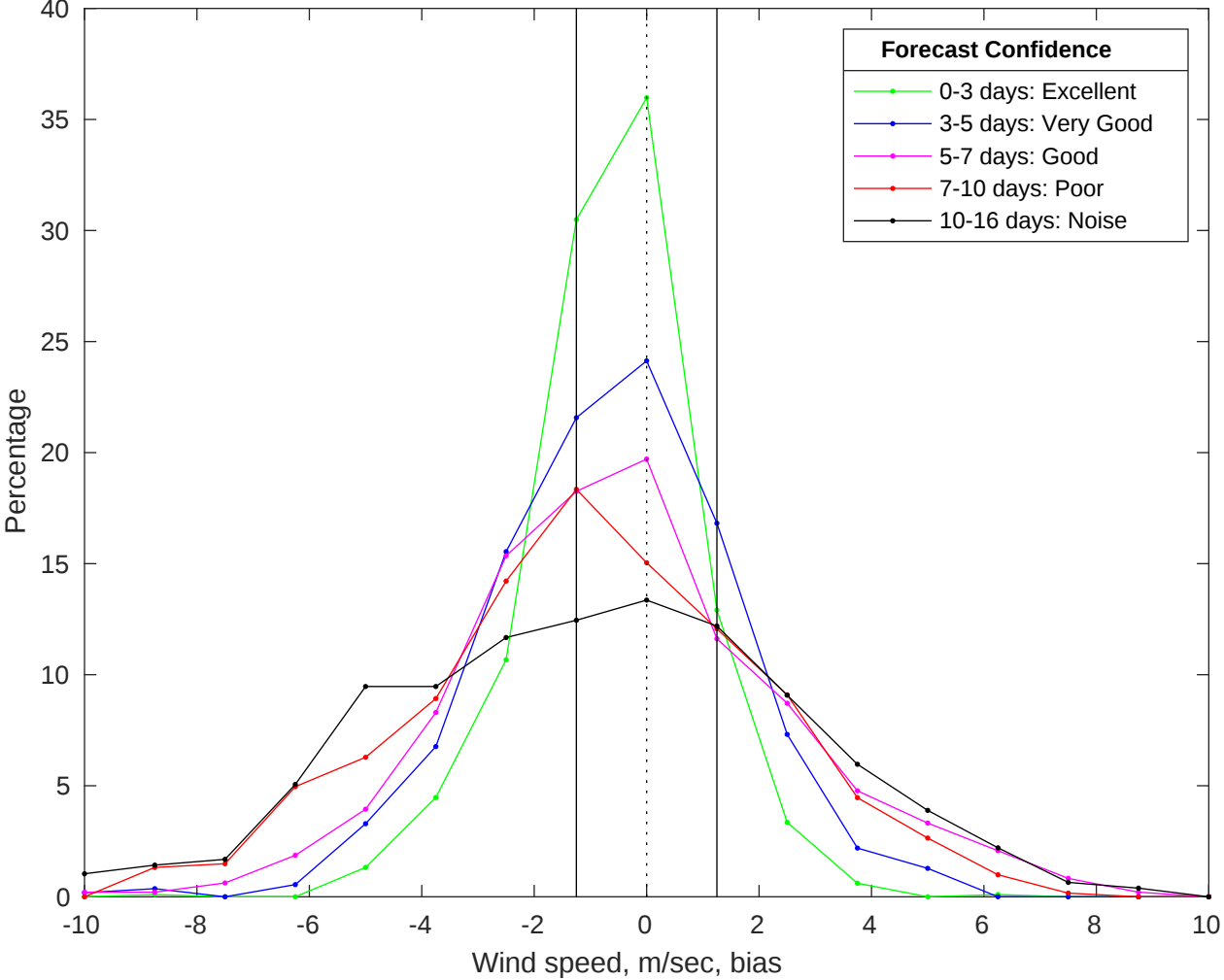
NDBC 42040 vs GFS Winds Bias Histogram: 21-Jan-2026
