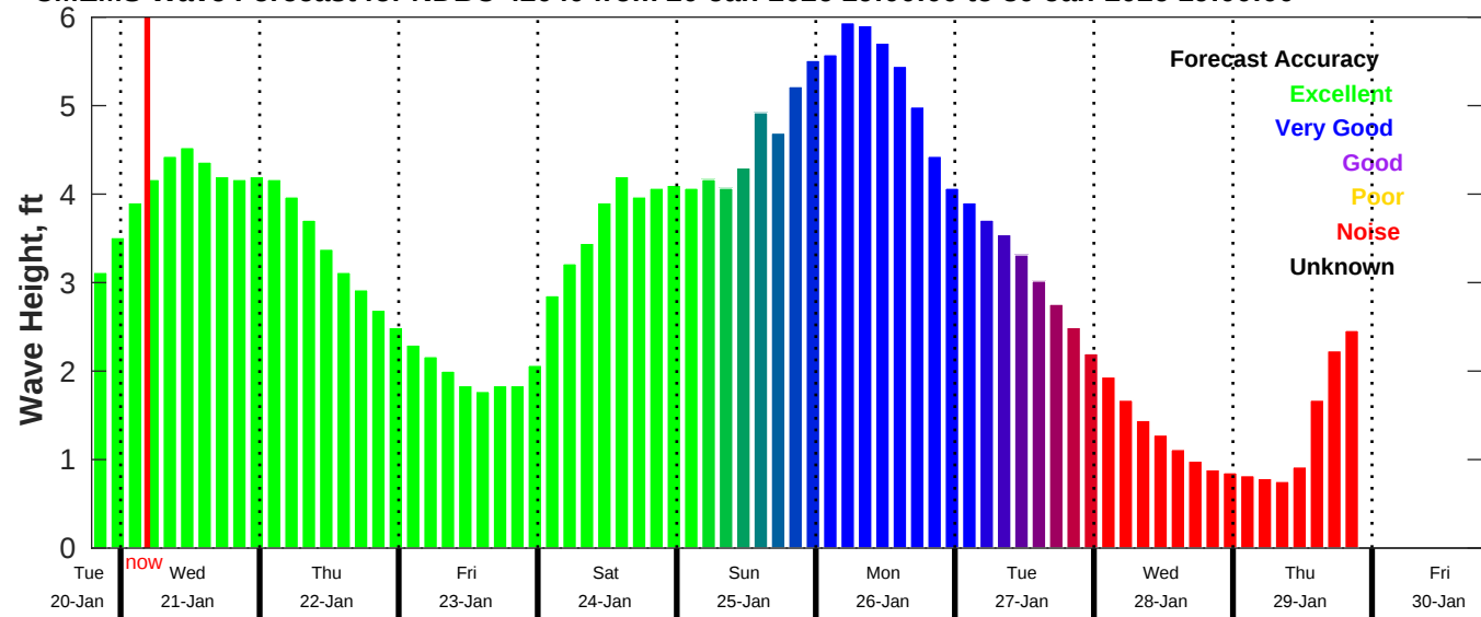
CMEMS Wave Forecast for NDBC 42040 from 20-Jan-2026 19:00:00 to 30-Jan-2026 19:00:00
