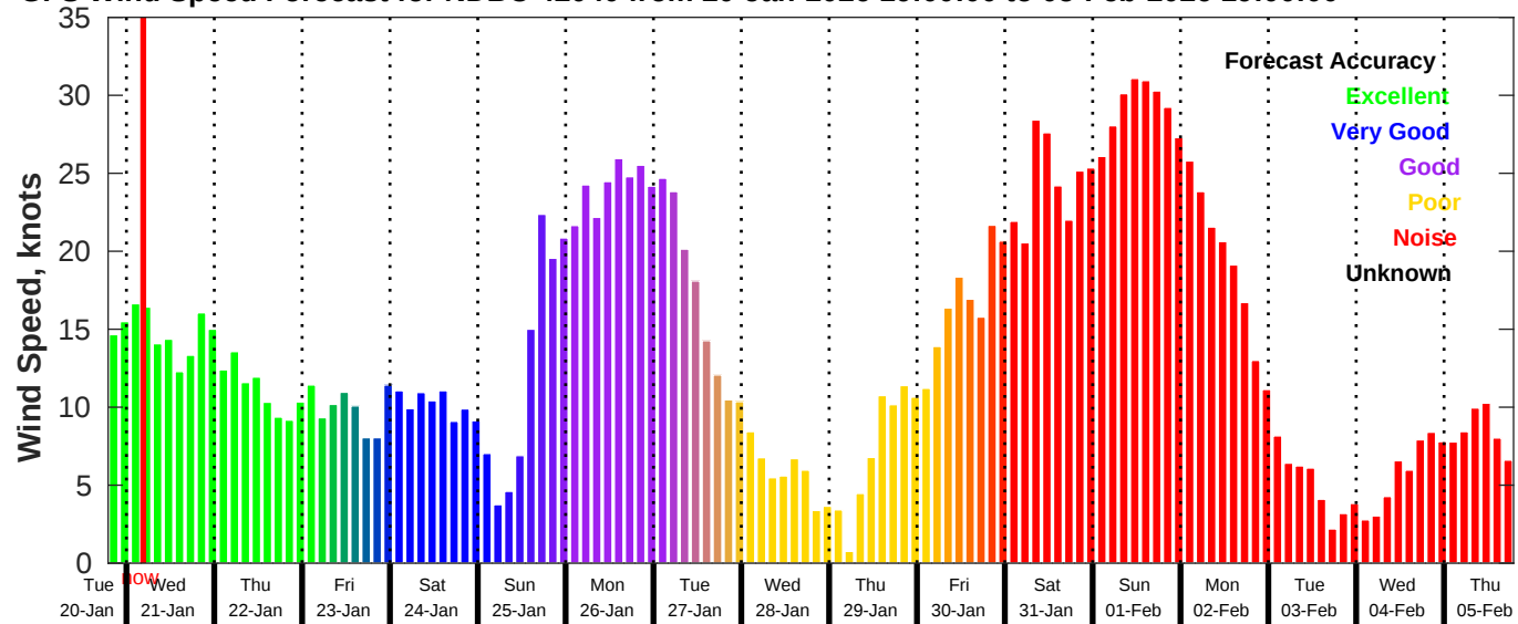
GFS Wind Speed Forecast for NDBC 42040 from 20-Jan-2026 19:00:00 to 05-Feb-2026 19:00:00
