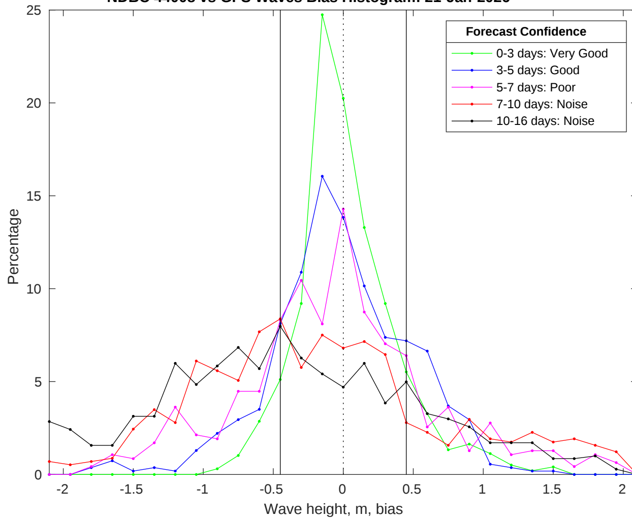
NDBC 44008 vs GFS Waves Bias Histogram: 21-Jan-2026
