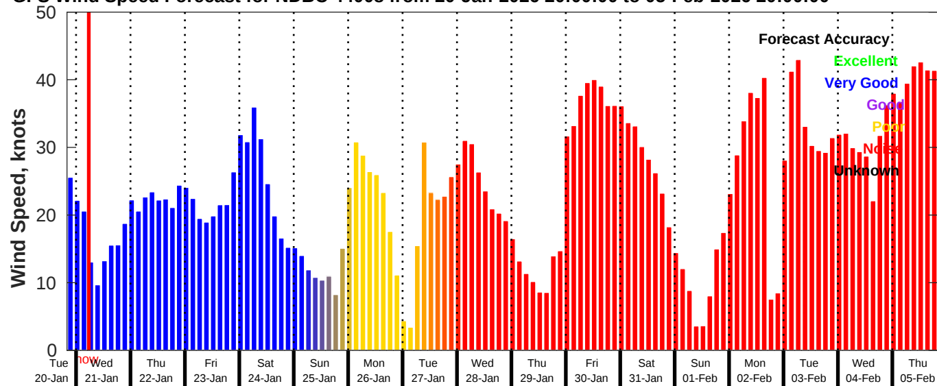
GFS Wind Speed Forecast for NDBC 44008 from 20-Jan-2026 20:00:00 to 05-Feb-2026 20:00:00
