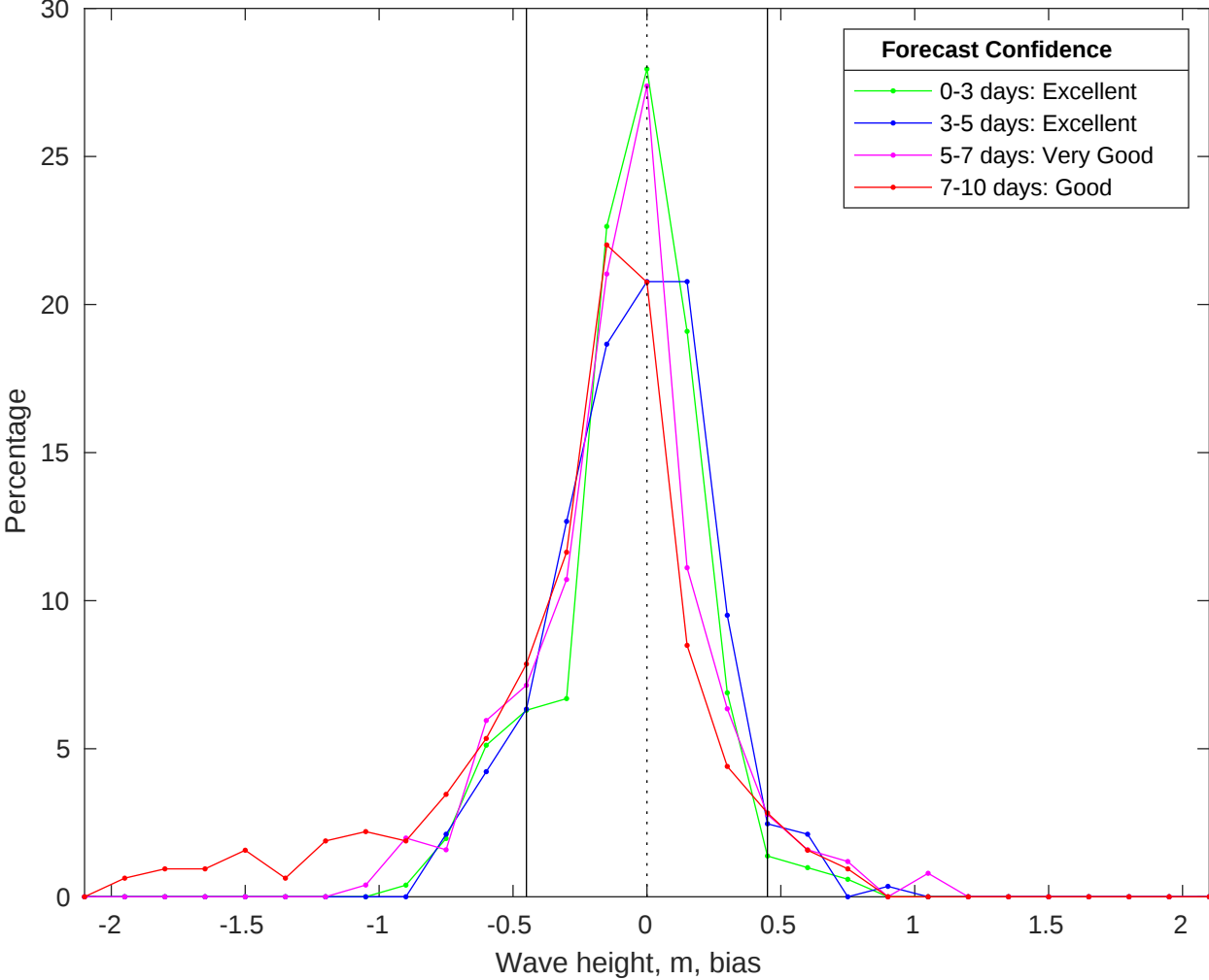
NDBC 46011 vs CMEMS Waves Bias Histogram: 21-Jan-2026
