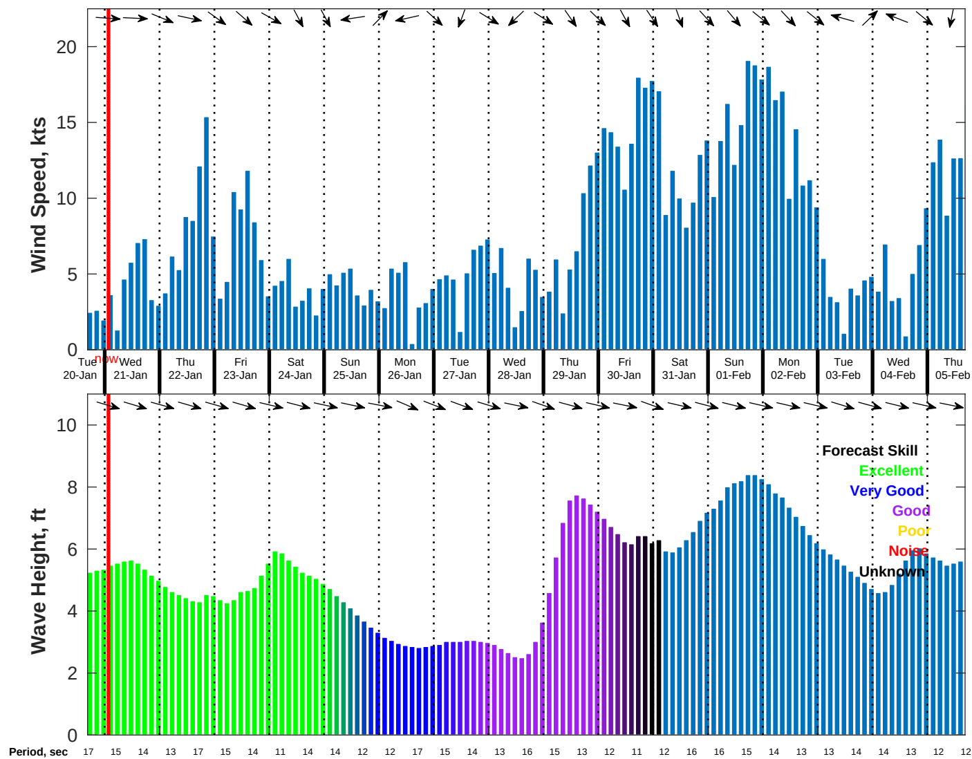
Wind & Wave Forecast for NDBC 46011 from 20-Jan-2026 16:00:00 to 05-Feb-2026 16:00:00
