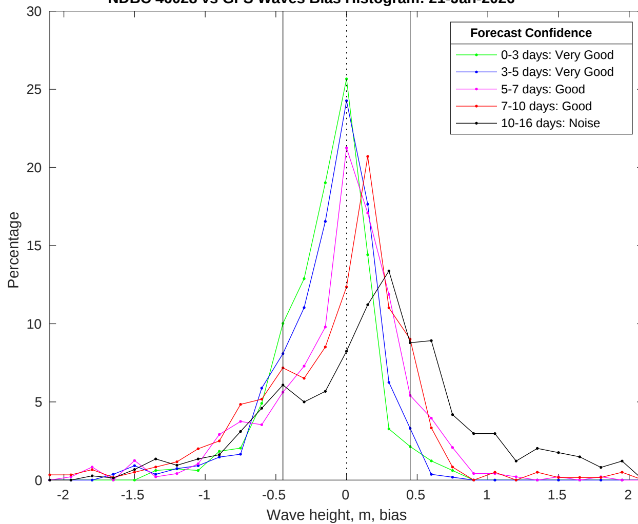
NDBC 46028 vs GFS Waves Bias Histogram: 21-Jan-2026
