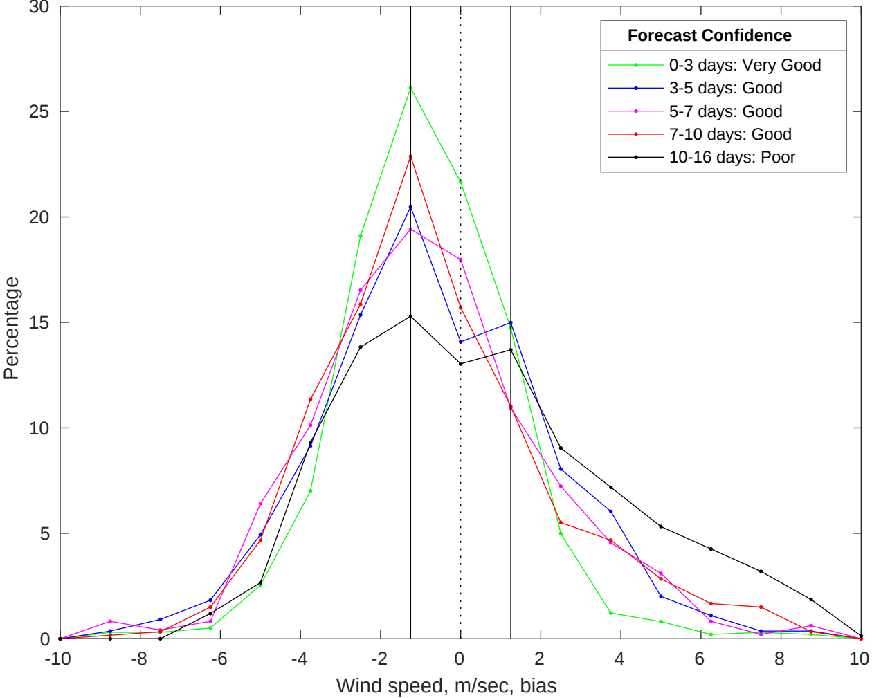
NDBC 46028 vs GFS Winds Bias Histogram: 21-Jan-2026
