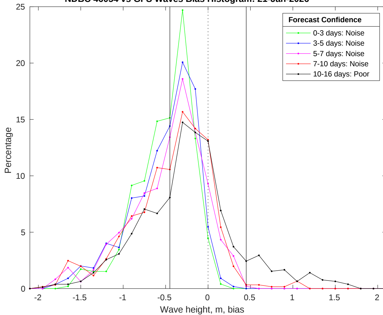
NDBC 46054 vs GFS Waves Bias Histogram: 21-Jan-2026
