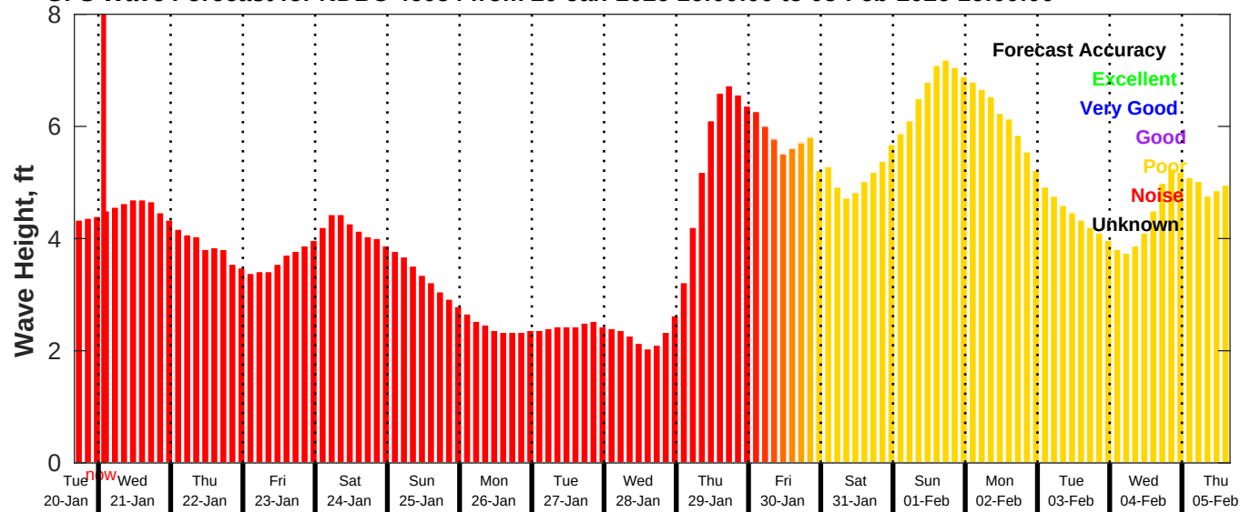
GFS Wave Forecast for NDBC 46054 from 20-Jan-2026 16:00:00 to 05-Feb-2026 16:00:00
