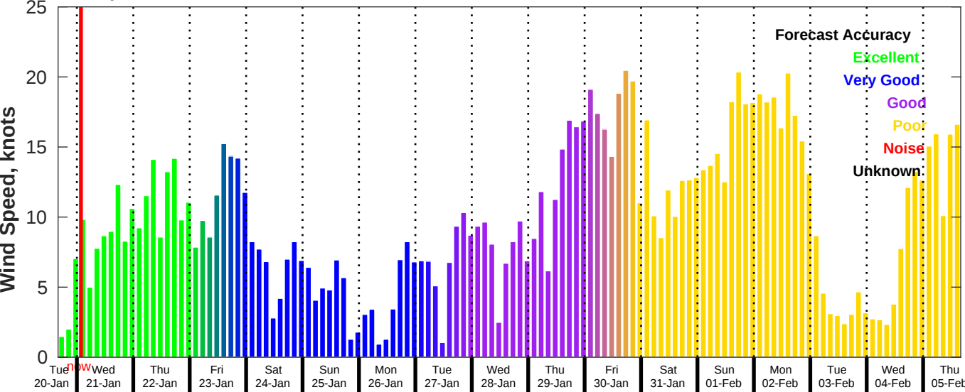
GFS Wind Speed Forecast for NDBC 46054 from 20-Jan-2026 16:00:00 to 05-Feb-2026 16:00:00
