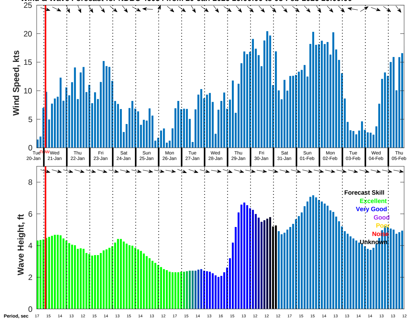
Wind & Wave Forecast for NDBC 46054 from 20-Jan-2026 16:00:00 to 05-Feb-2026 16:00:00
