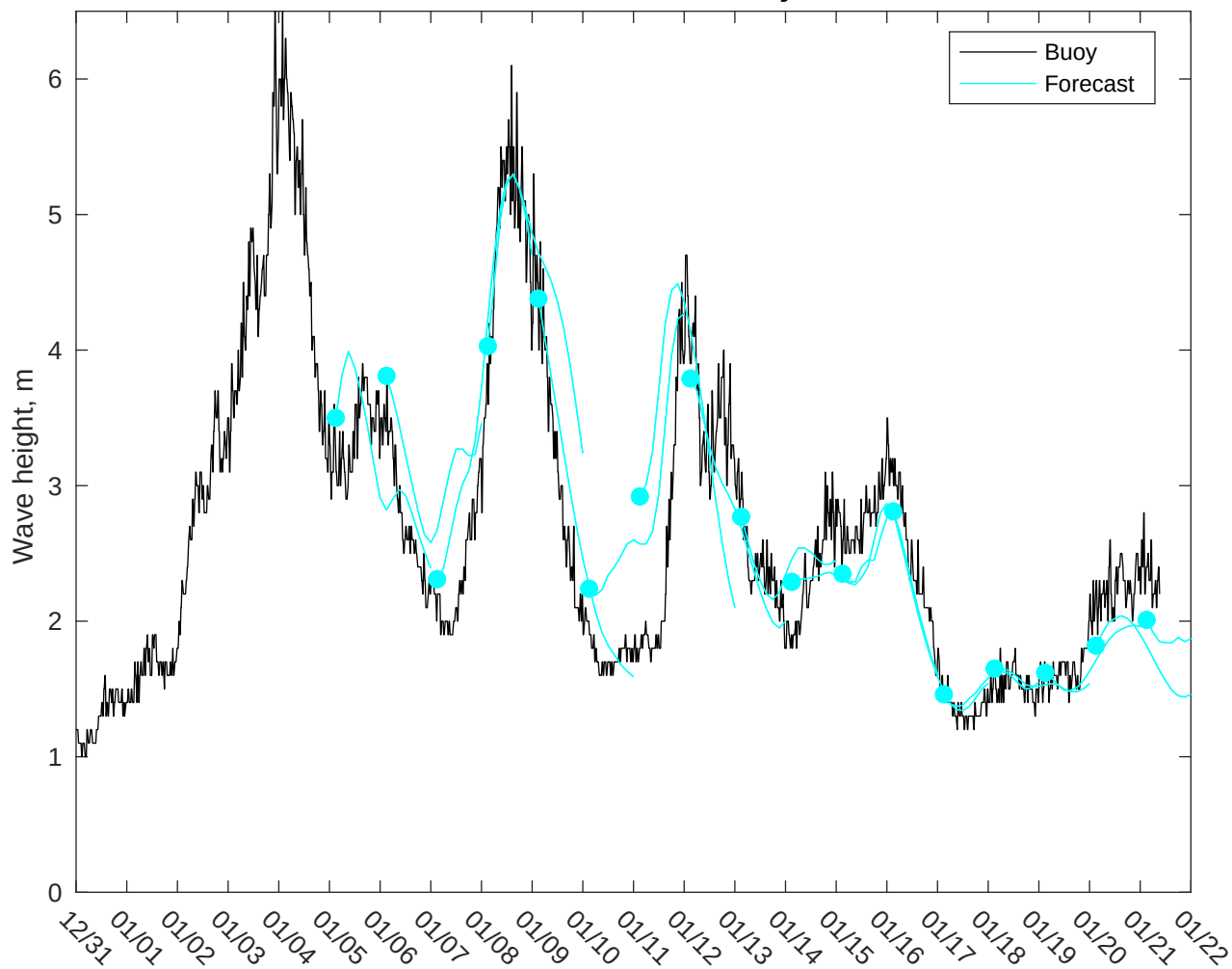
NDBC 46059 vs CMEMS Waves: 5 to 7 day forecast
