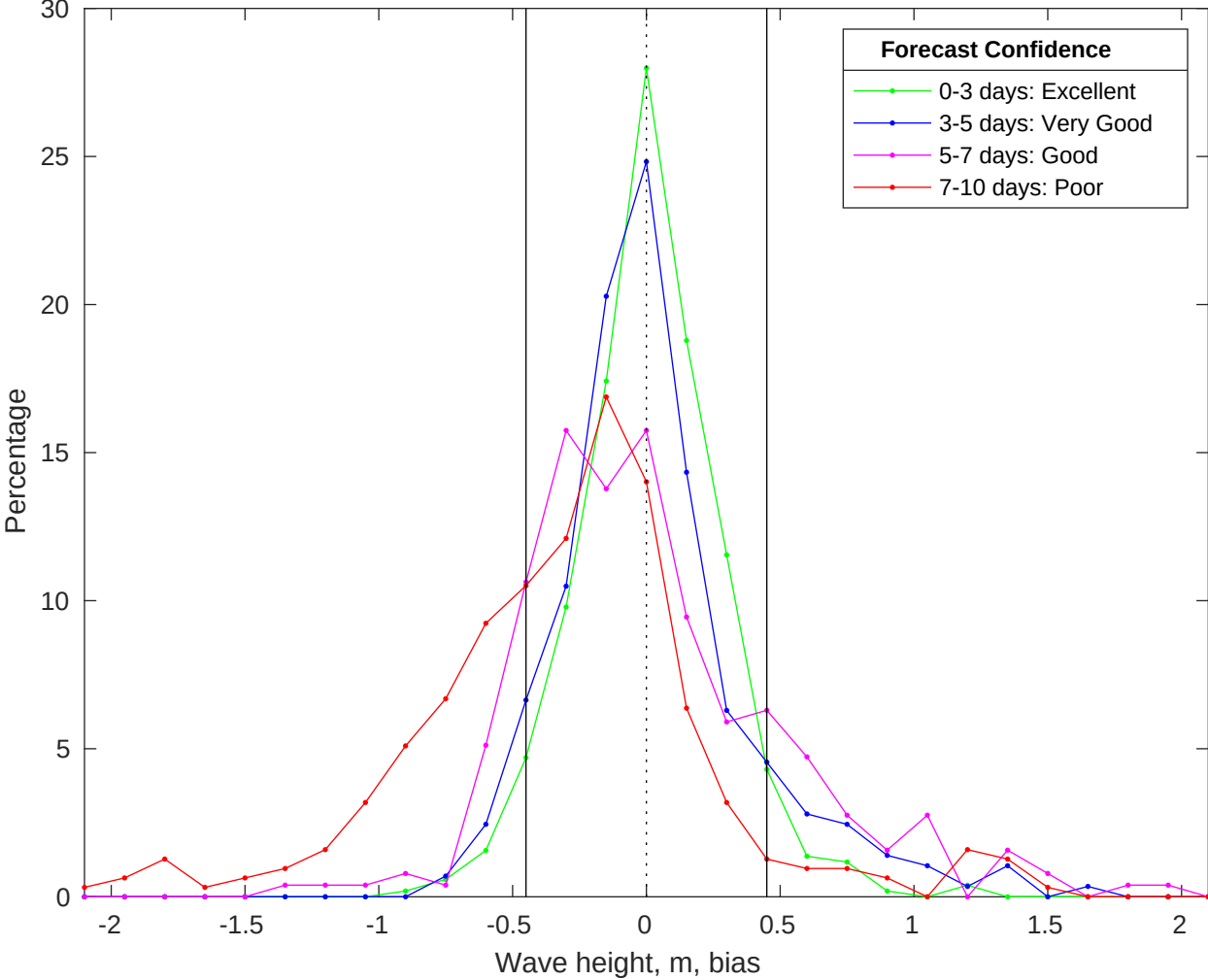
NDBC 46059 vs CMEMS Waves Bias Histogram: 21-Jan-2026
