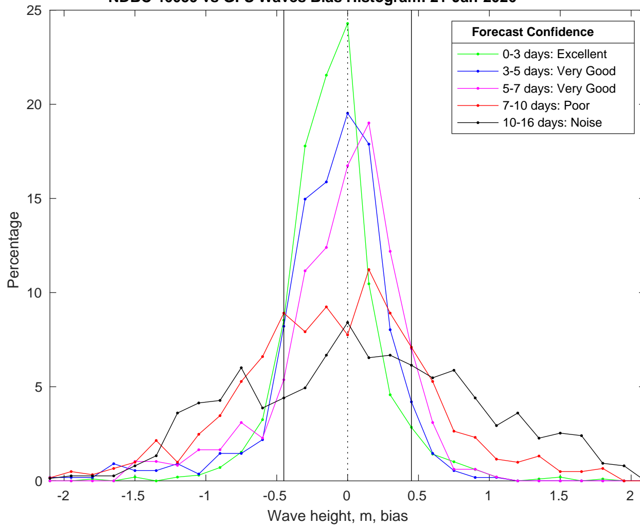
NDBC 46059 vs GFS Waves Bias Histogram: 21-Jan-2026
