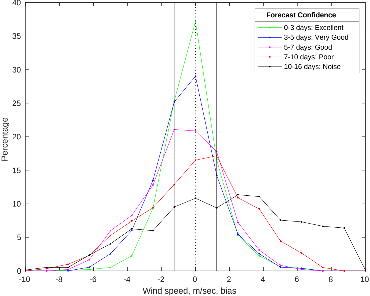
NDBC 46059 vs GFS Winds Bias Histogram: 21-Jan-2026
