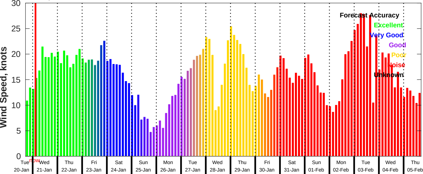
GFS Wind Speed Forecast for NDBC 46059 from 20-Jan-2026 17:00:00 to 05-Feb-2026 17:00:00
