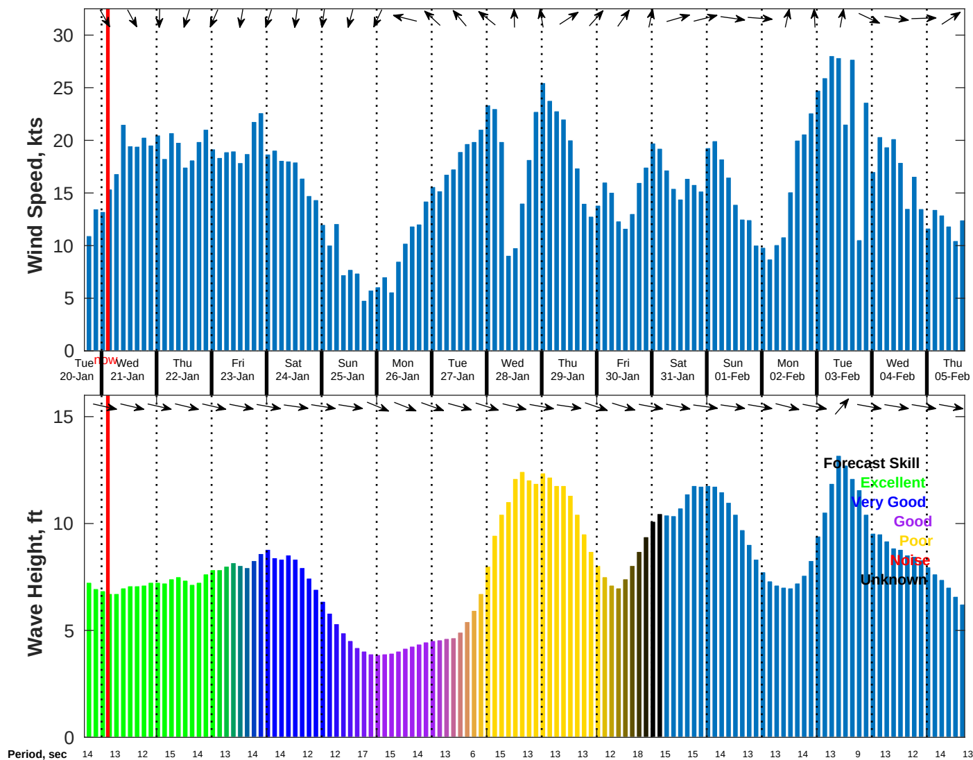
Wind & Wave Forecast for NDBC 46059 from 20-Jan-2026 17:00:00 to 05-Feb-2026 17:00:00
