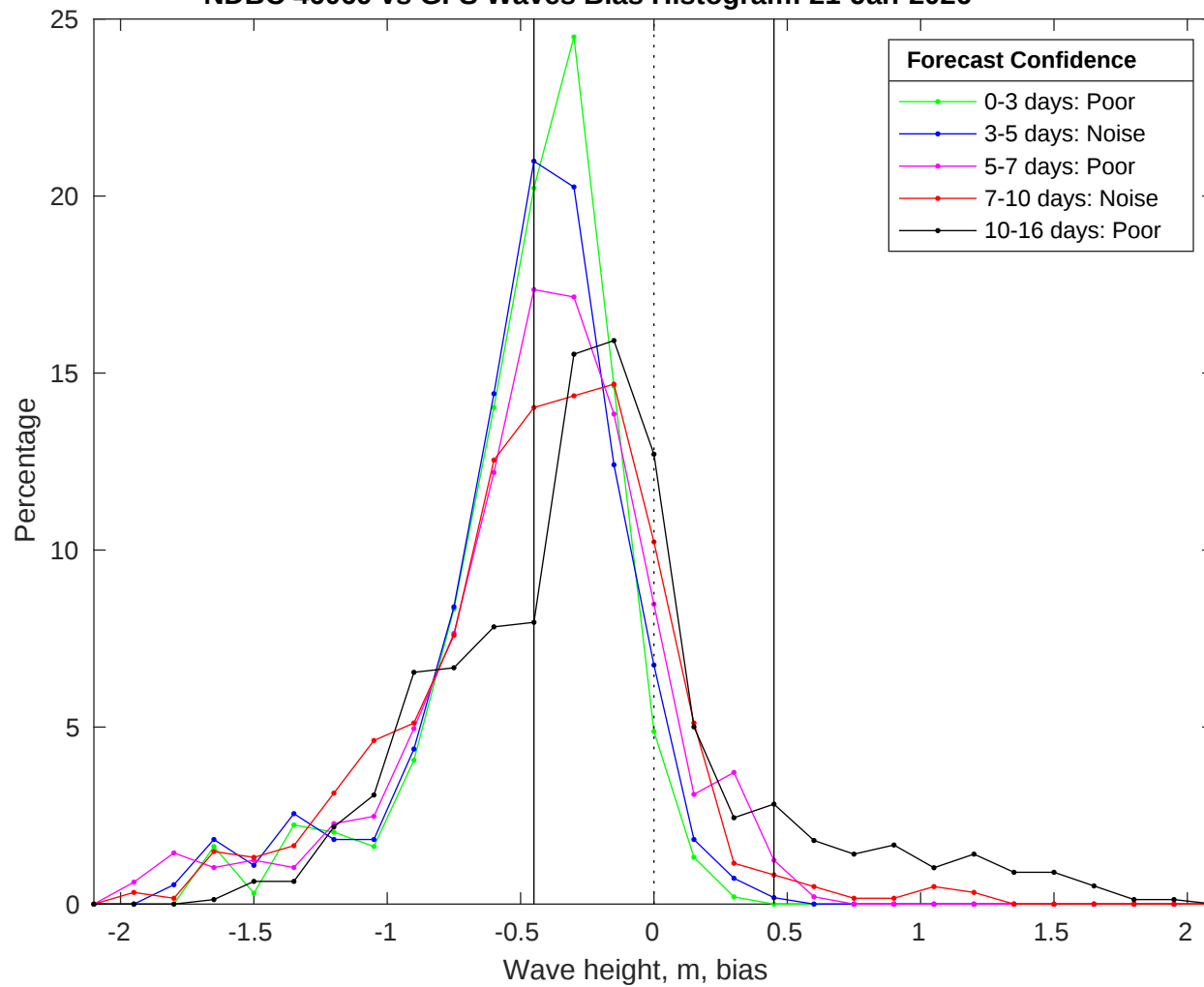
NDBC 46069 vs GFS Waves Bias Histogram: 21-Jan-2026
