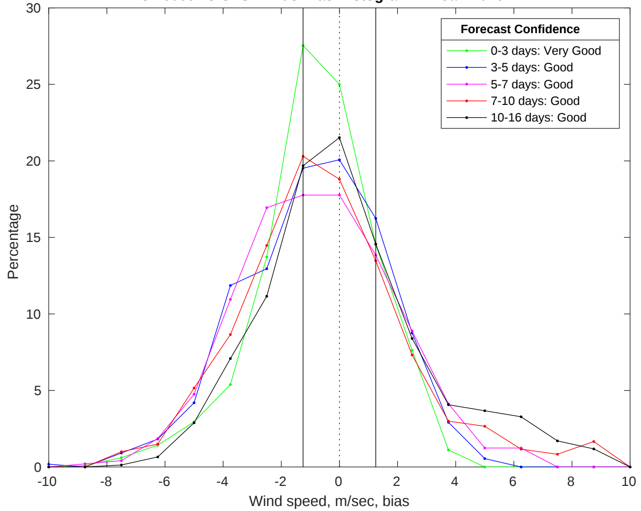
NDBC 46069 vs GFS Winds Bias Histogram: 21-Jan-2026
