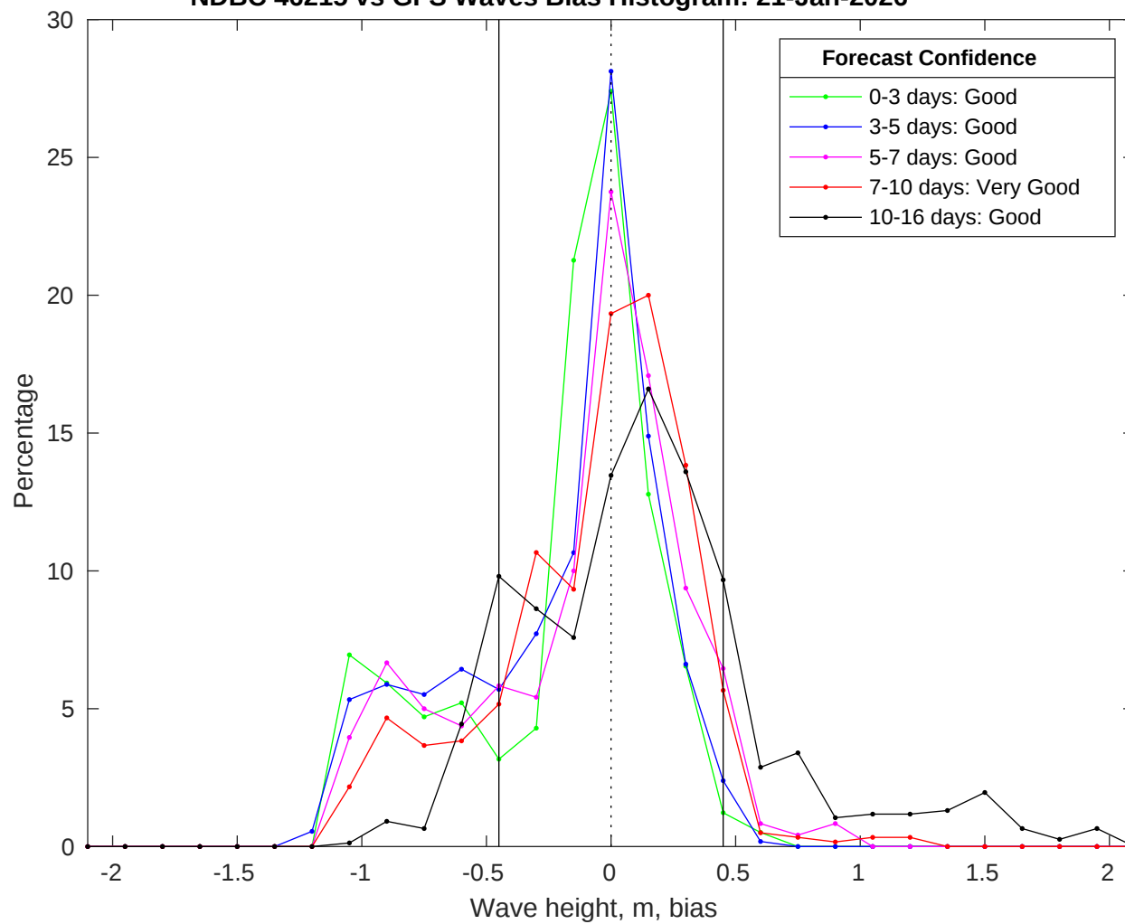
NDBC 46215 vs GFS Waves Bias Histogram: 21-Jan-2026
