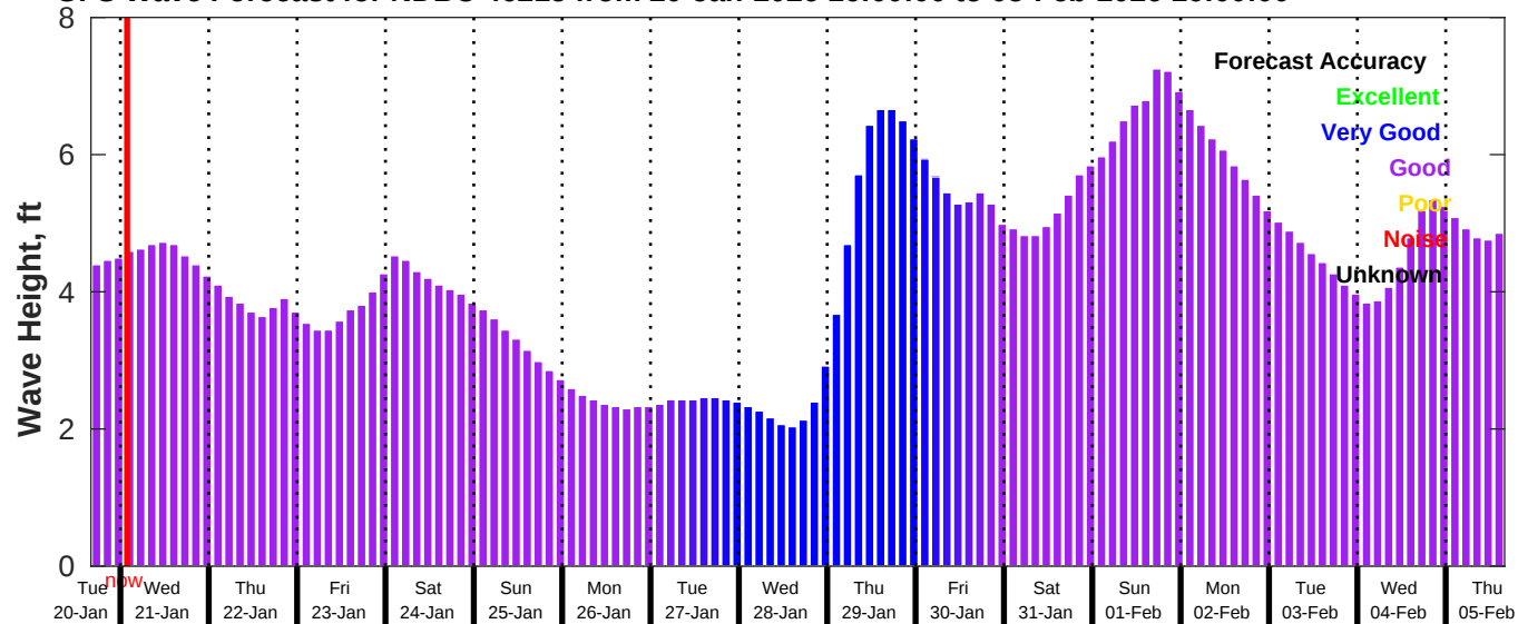
GFS Wave Forecast for NDBC 46215 from 20-Jan-2026 16:00:00 to 05-Feb-2026 16:00:00
