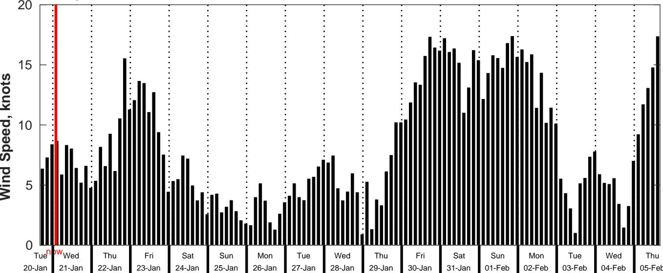
GFS Wind Speed Forecast for NDBC 46259 from 20-Jan-2026 16:00:00 to 05-Feb-2026 16:00:00
