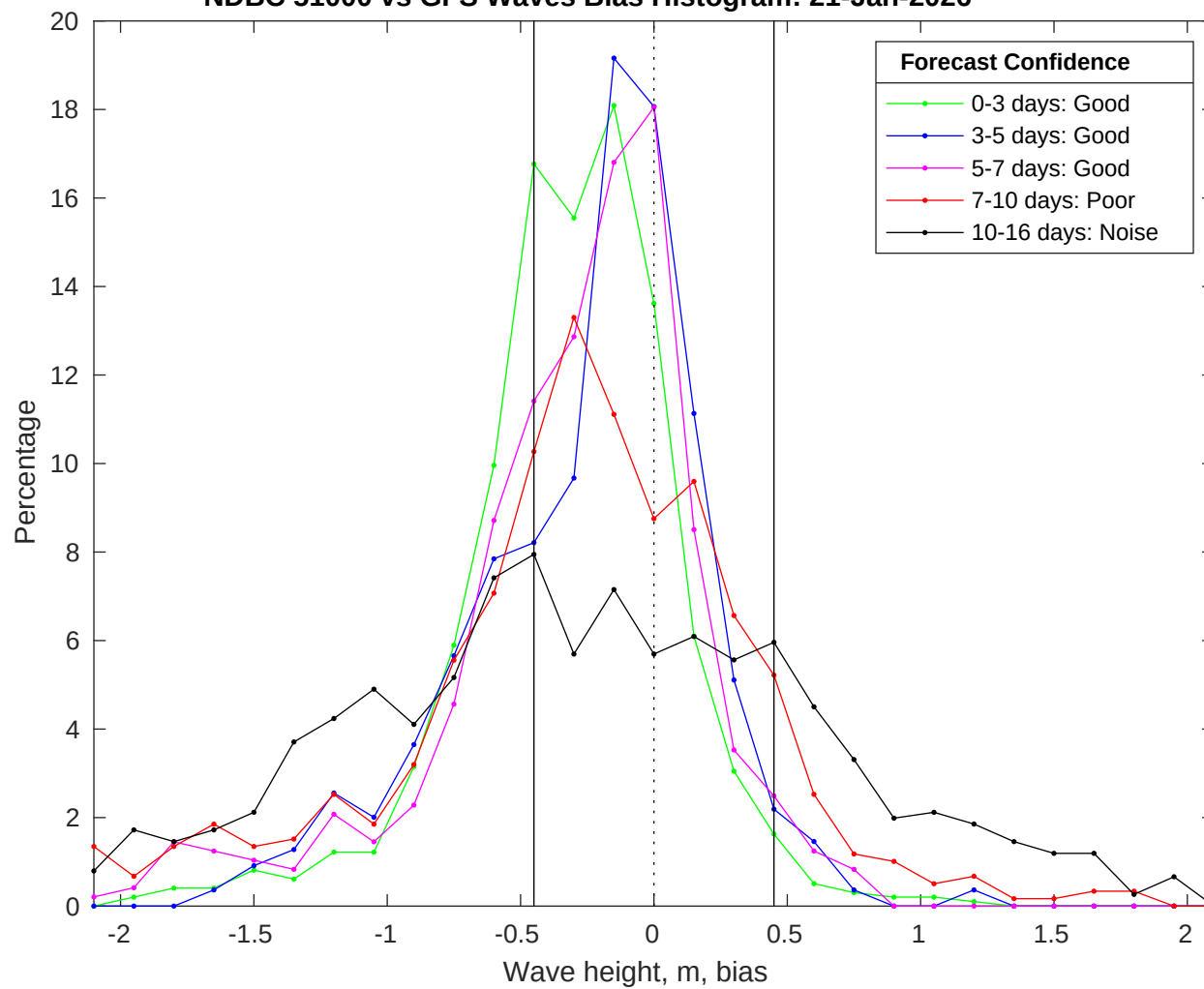
NDBC 51000 vs GFS Waves Bias Histogram: 21-Jan-2026
