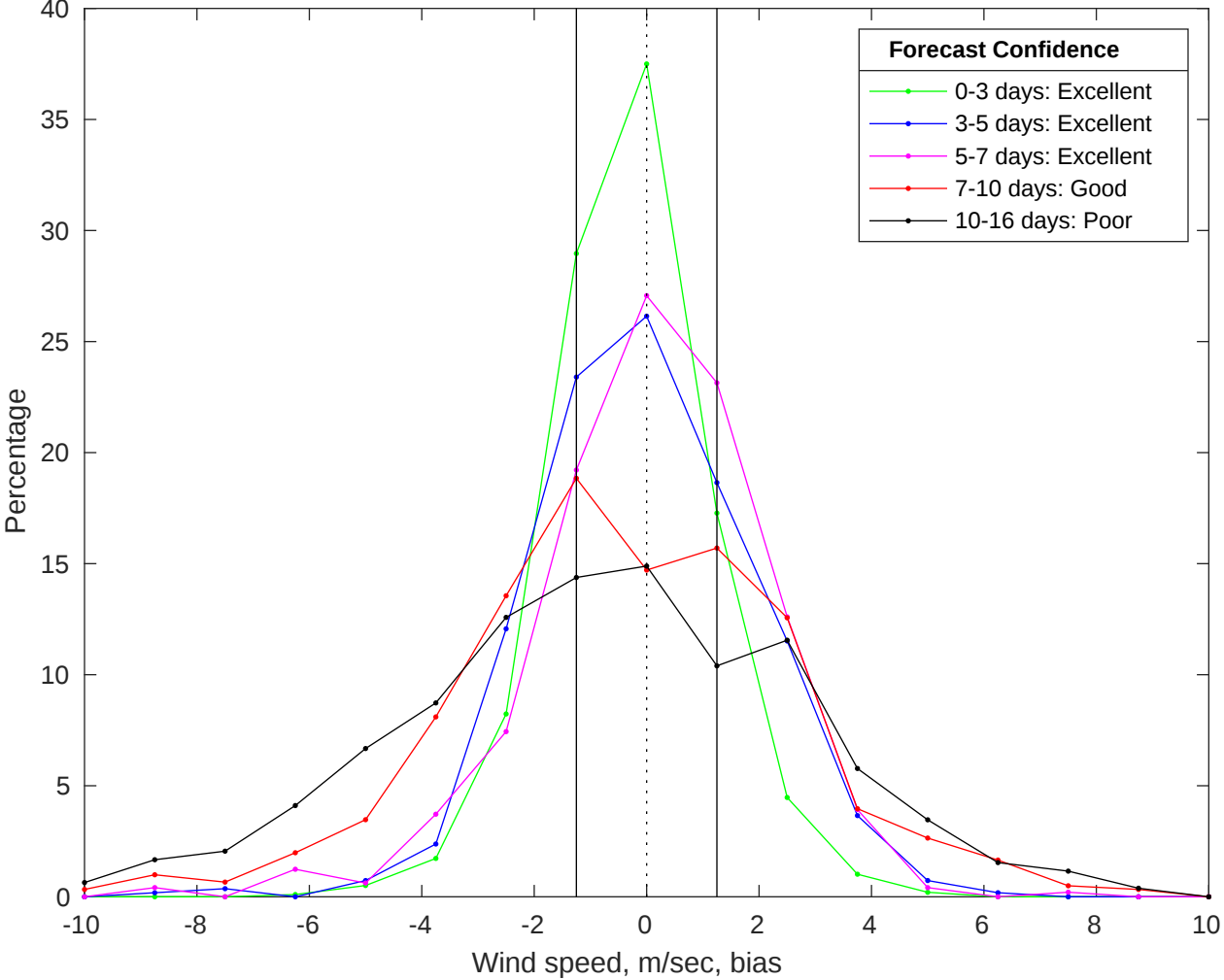
NDBC 51000 vs GFS Winds Bias Histogram: 21-Jan-2026
