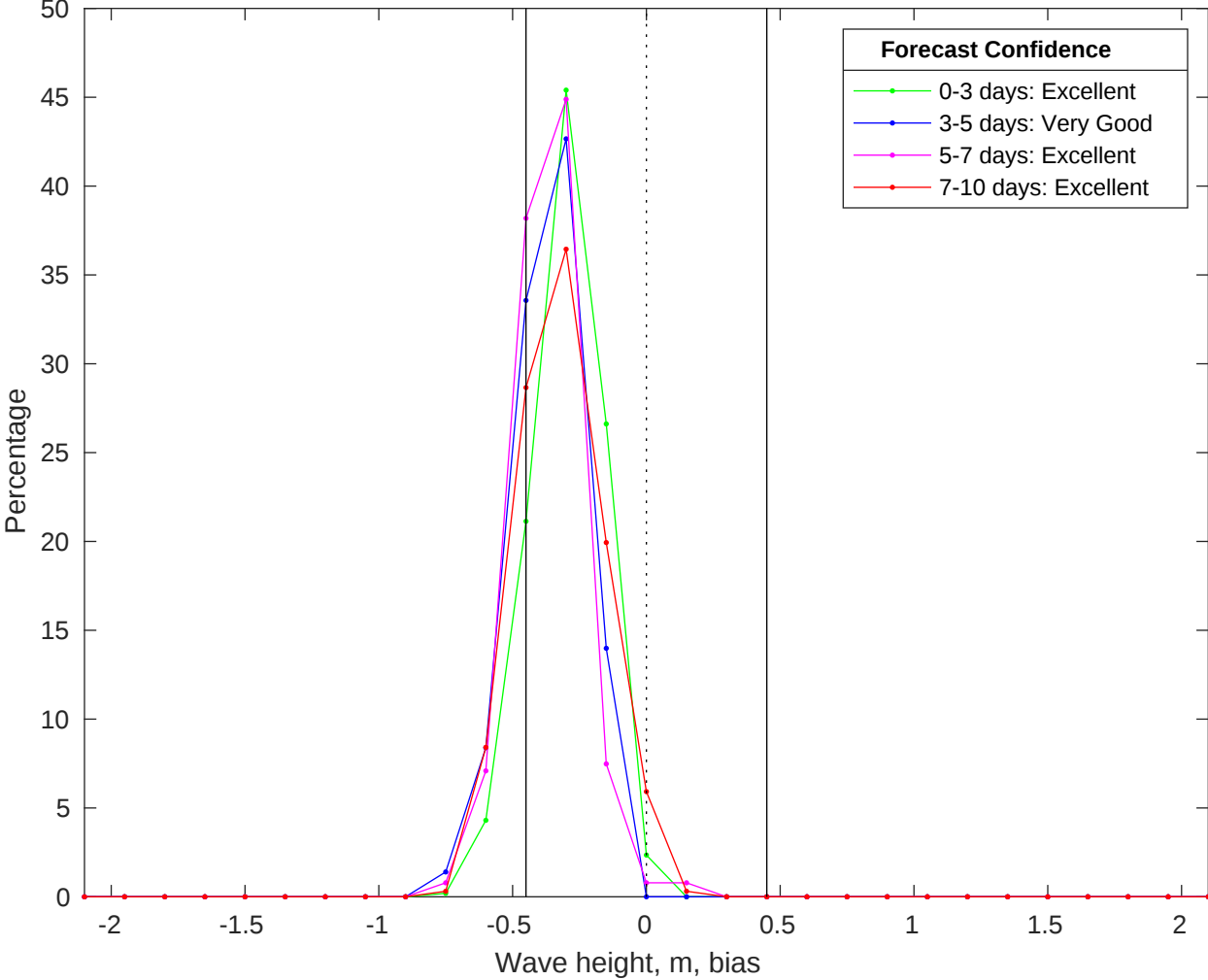
NDBC 51209 vs CMEMS Waves Bias Histogram: 21-Jan-2026
