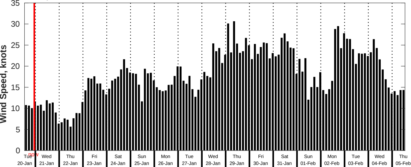
GFS Wind Speed Forecast for NDBC 51209 from 20-Jan-2026 13:00:00 to 05-Feb-2026 13:00:00
