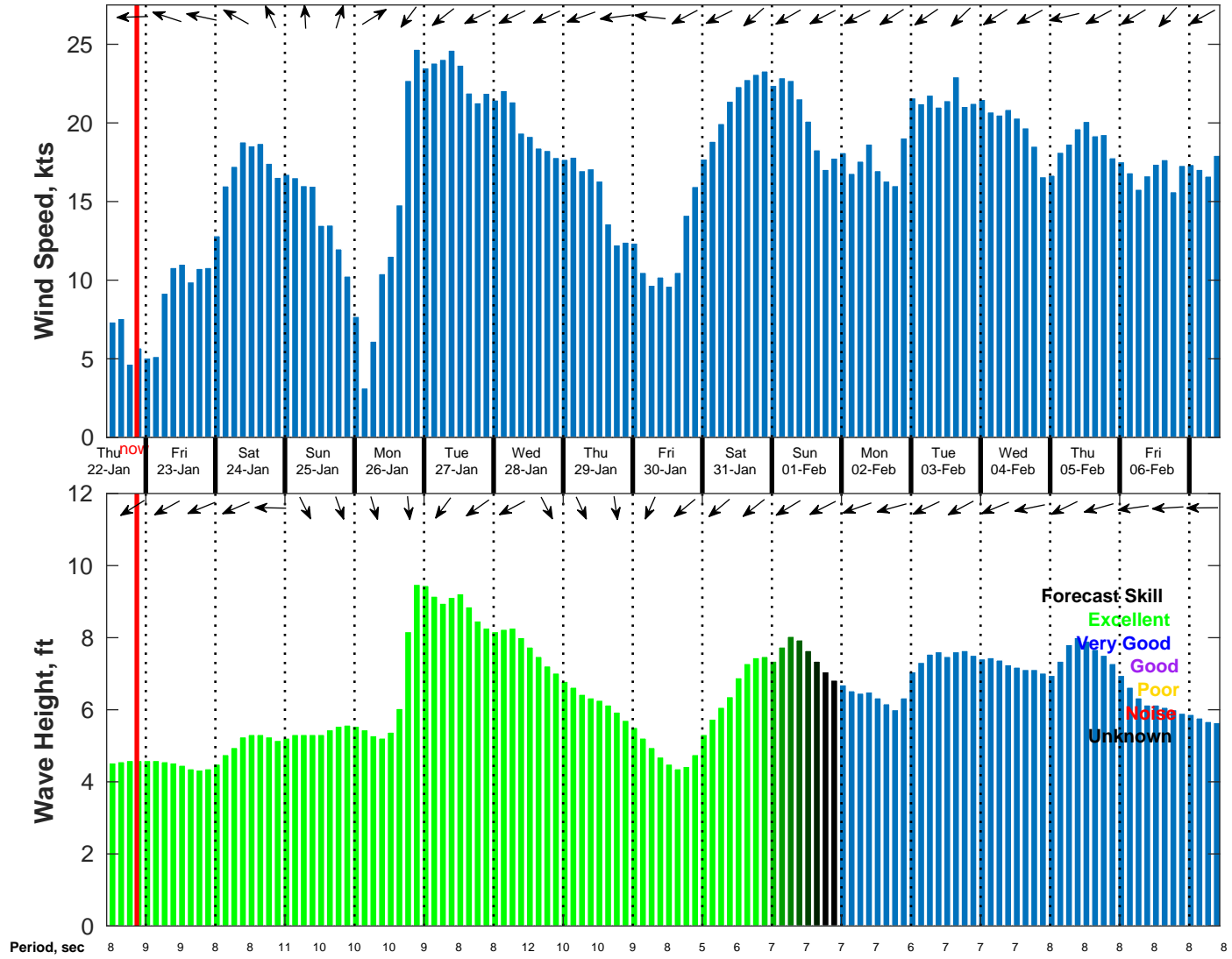
Wind & Wave Forecast for NDBC 52211 from 21-Jan-2026 11:00:00 to 06-Feb-2026 11:00:00
