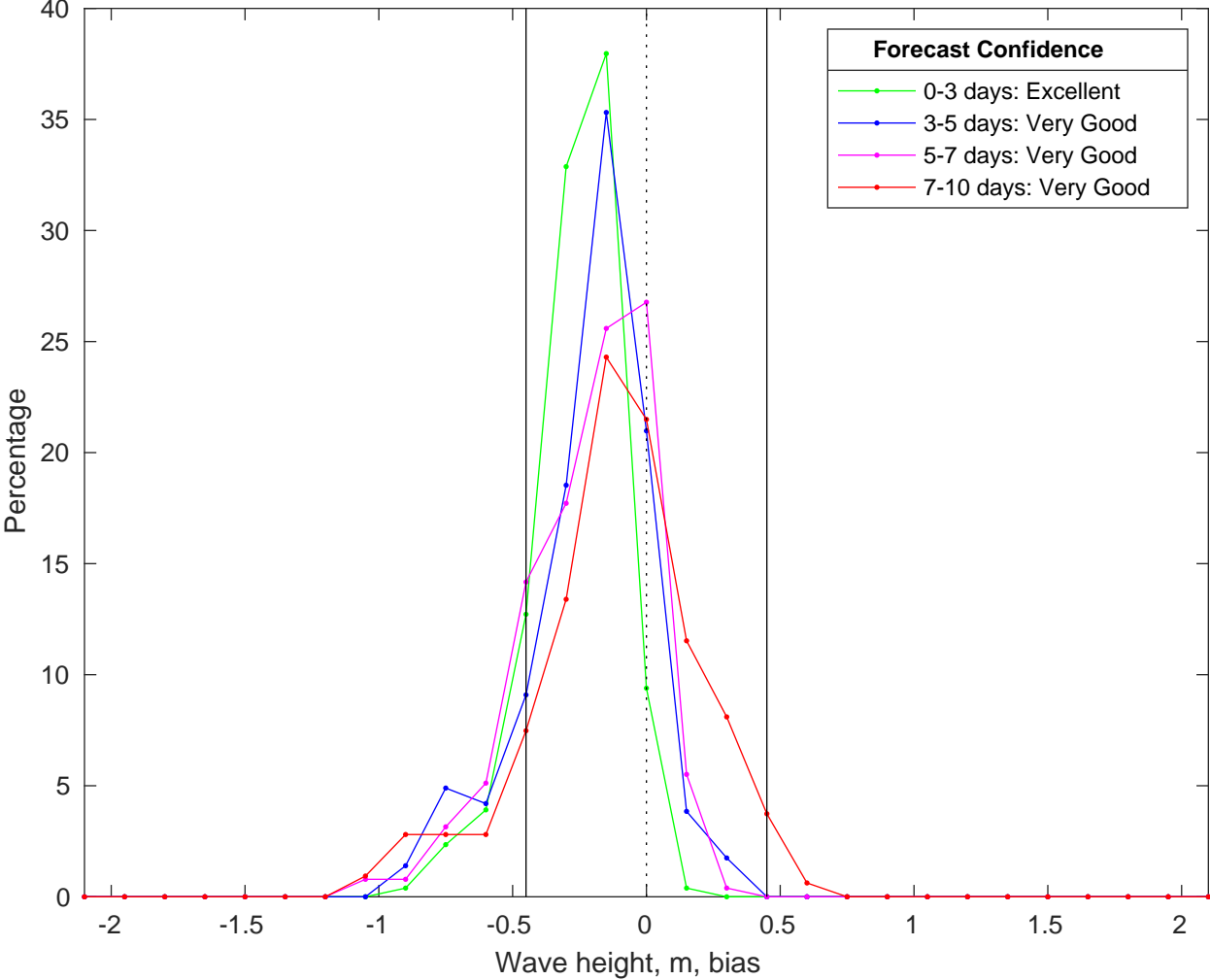
NDBC 52213 vs CMEMS Waves Bias Histogram: 21-Jan-2026
