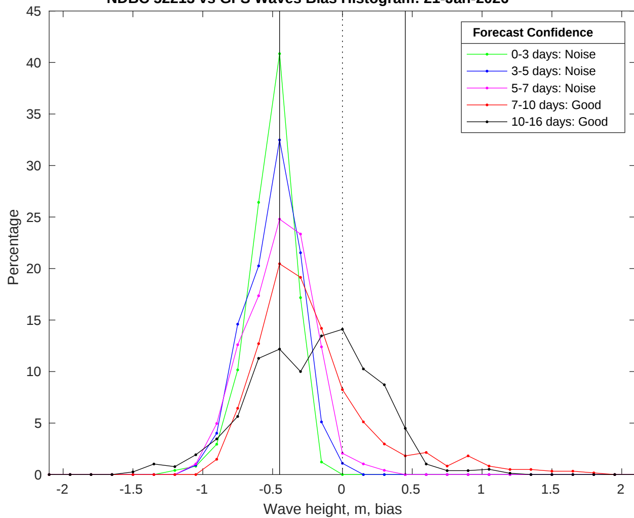
NDBC 52213 vs GFS Waves Bias Histogram: 21-Jan-2026
