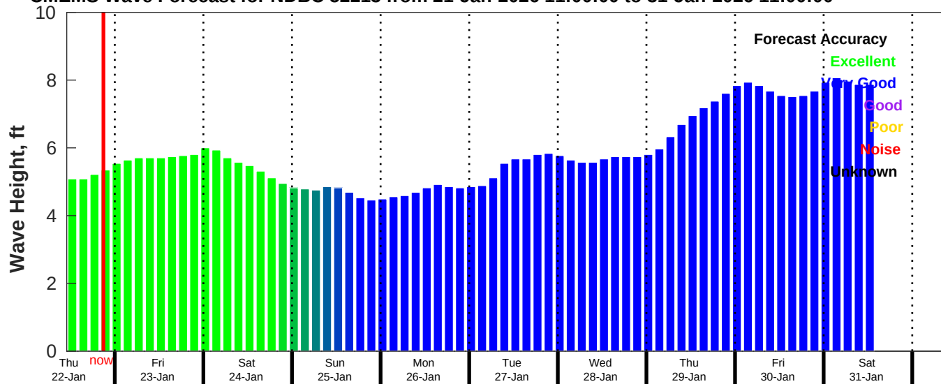
CMEMS Wave Forecast for NDBC 52213 from 21-Jan-2026 11:00:00 to 31-Jan-2026 11:00:00
