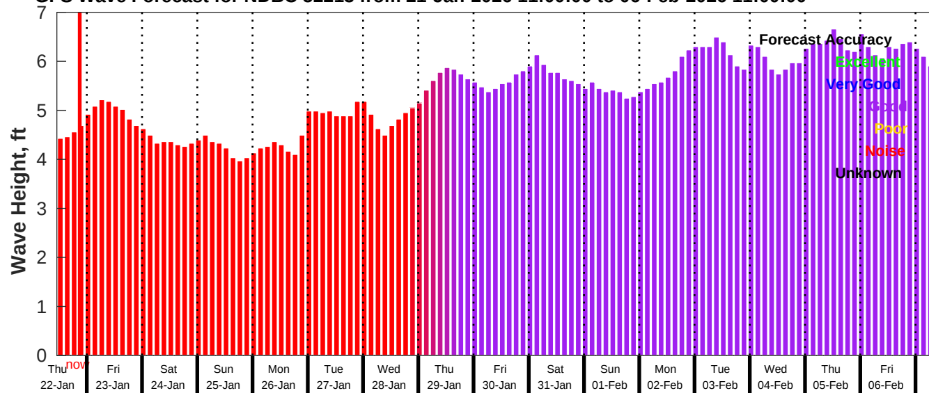
GFS Wave Forecast for NDBC 52213 from 21-Jan-2026 11:00:00 to 06-Feb-2026 11:00:00
