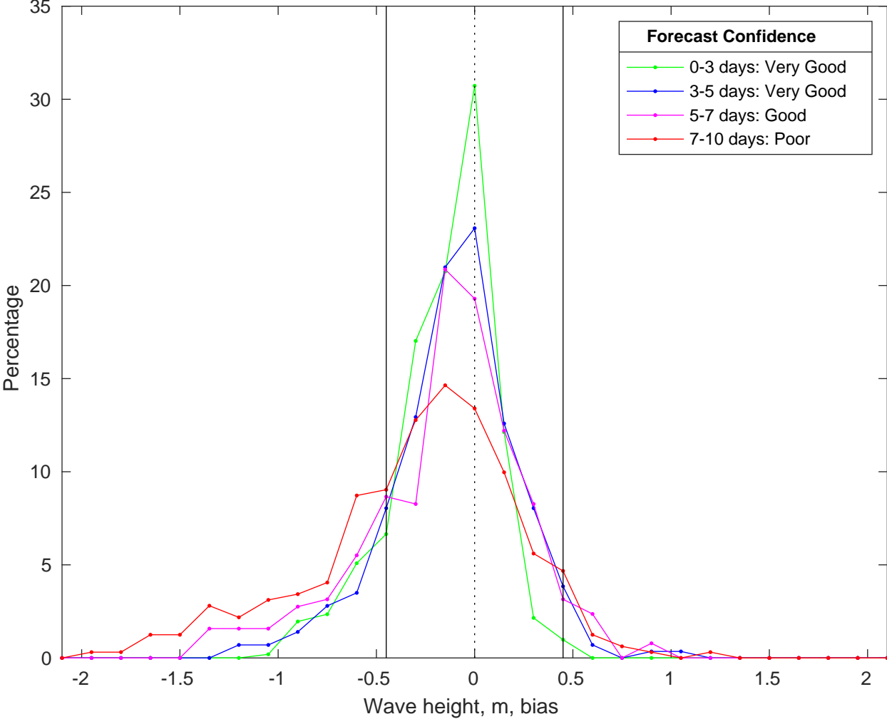
NDBC 41004 vs CMEMS Waves Bias Histogram: 22-Jan-2026
