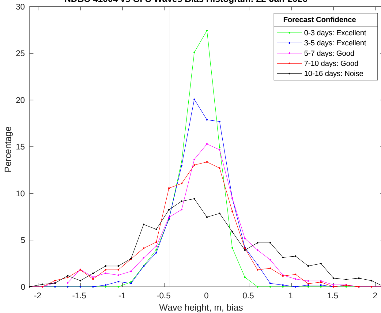
NDBC 41004 vs GFS Waves Bias Histogram: 22-Jan-2026
