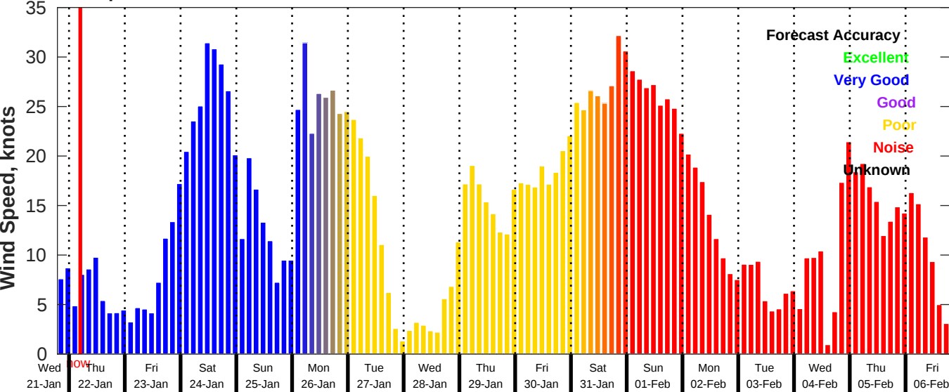
GFS Wind Speed Forecast for NDBC 41004 from 21-Jan-2026 19:00:00 to 06-Feb-2026 19:00:00
